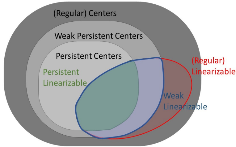
Fig. 1. The relation between the varieties V_c , V_{pc} , V_{wpc} and V_l , V_{\mathcal{L}^p} , V_{\mathcal{L}^{wp}} , V_{\mathcal{L}^p} \subset V_{\mathcal{L}^{wp}} \subset \mathbb{C}^{14} of the cubic system (7).
