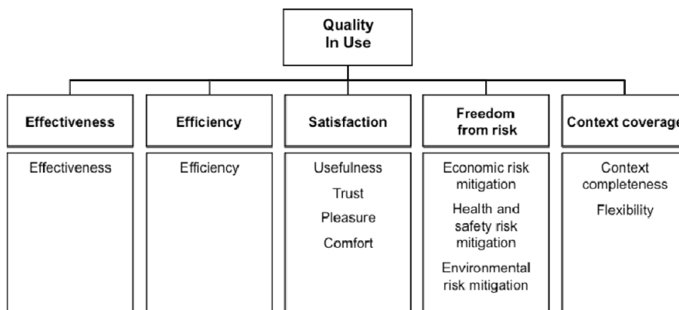
Figure 2.1: ISO/IEC 25010 – Quality in Use Model.
