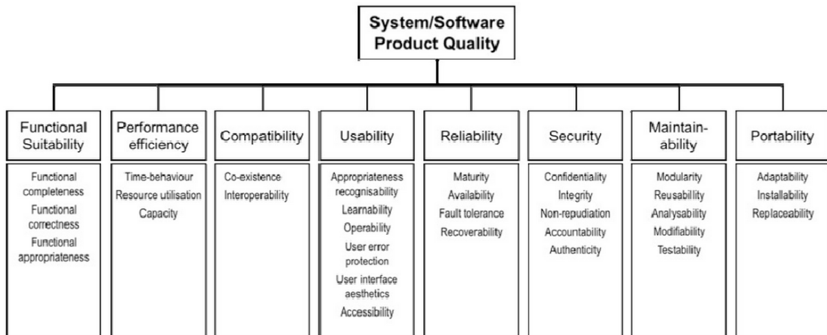
Figure 2.2: ISO/IEC 25010 – Product Quality Model.
